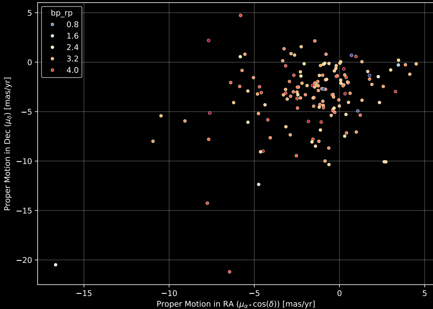
APOGEE DR17 Field: [357+02-O] Proper Motion Diagram (n= 153)
