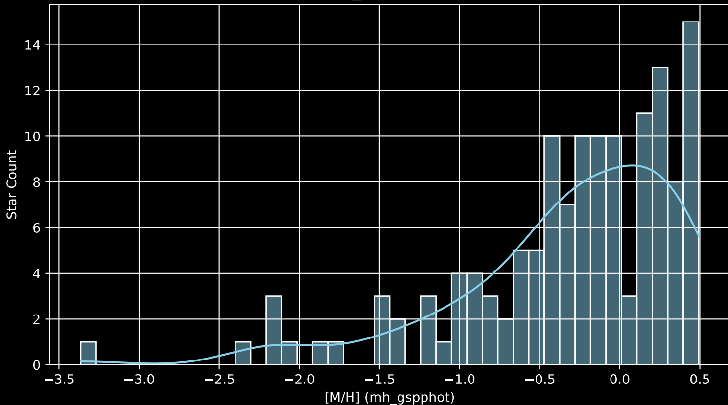
APOGEE DR17 Field: [357+02-O [M/H] (mh_gspphot) (n= 137)
