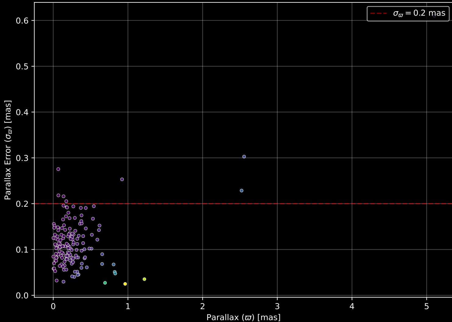
APOGEE DR17 Field: [357+02-O] Parallax Quality (n= 153)
