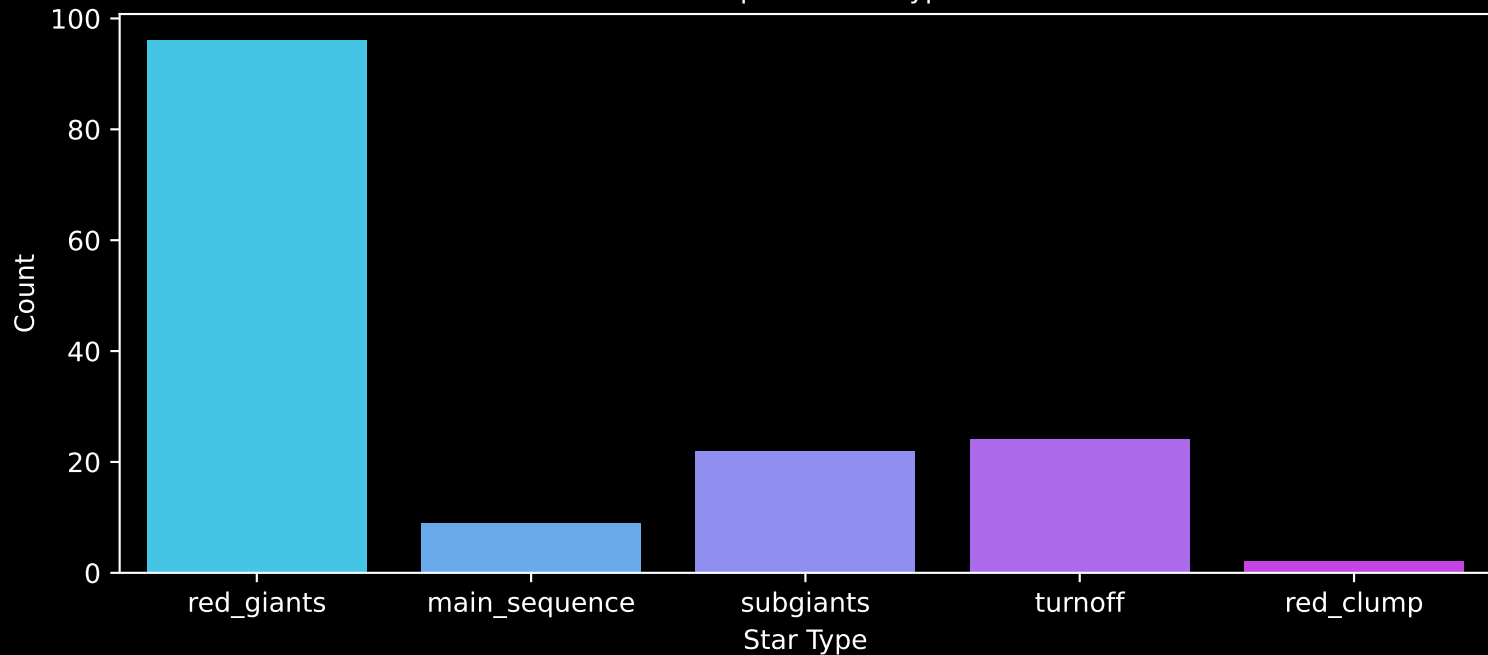
APOGEE DR17 Field: [357+02-O] Count plot of Star Type
