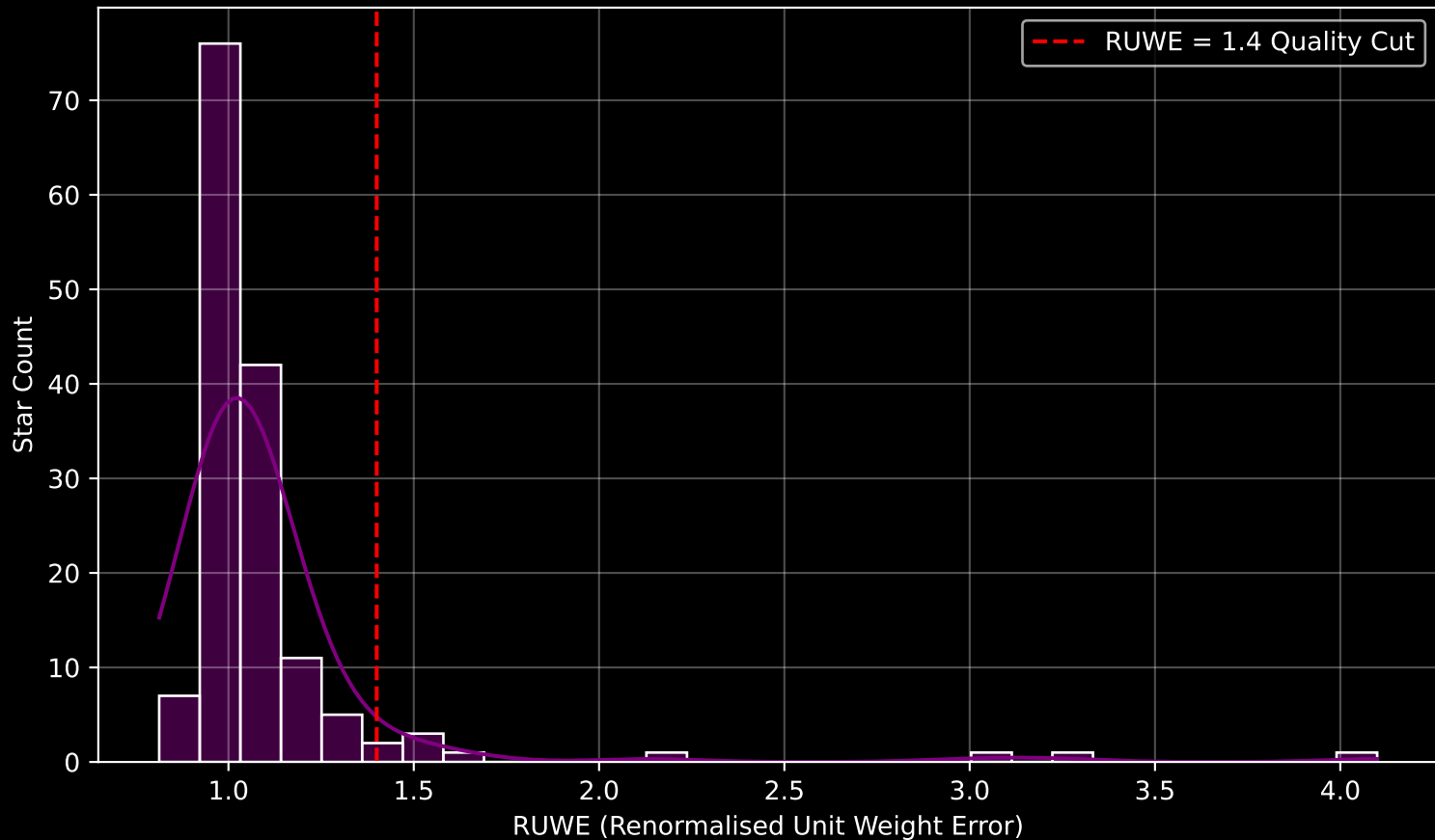
GAPOGEE DR17 Field [357+02-O] RUWE Distribution (n= 151)
