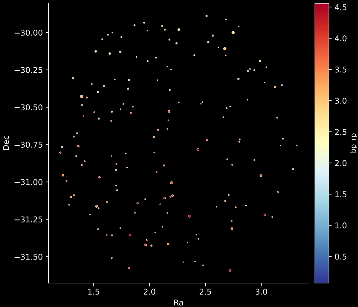
APOGEE DR17 Field: [357+02-O] Stars: 153
