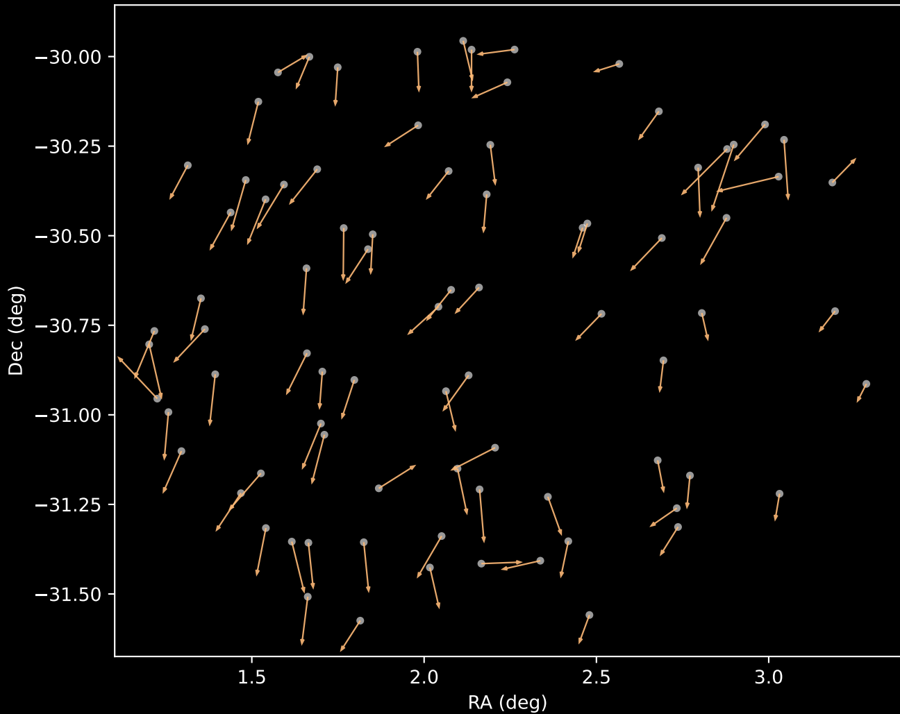
APOGEE DR17 Cluster 3 Proper Motion Vectors (n=83)
