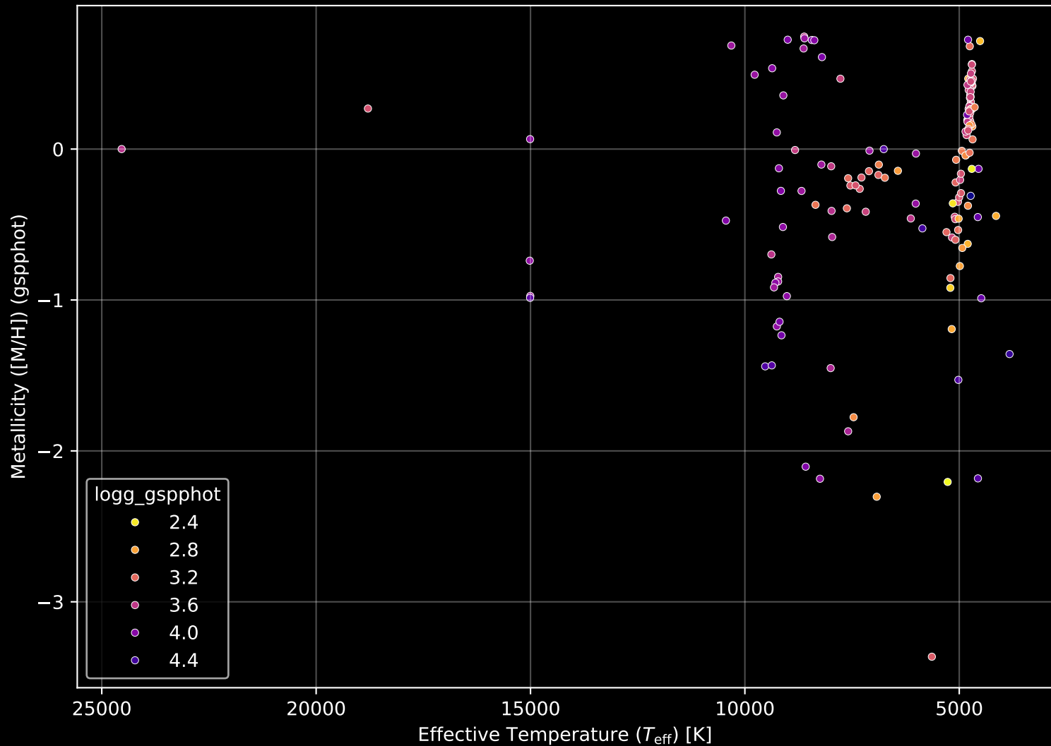
APOGEE DR17 Field: [357+02-O] Stellar Population Parameters (n= 153)
